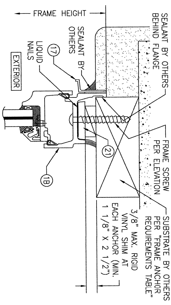
SECTION H SCALE: 1/2 FULL
